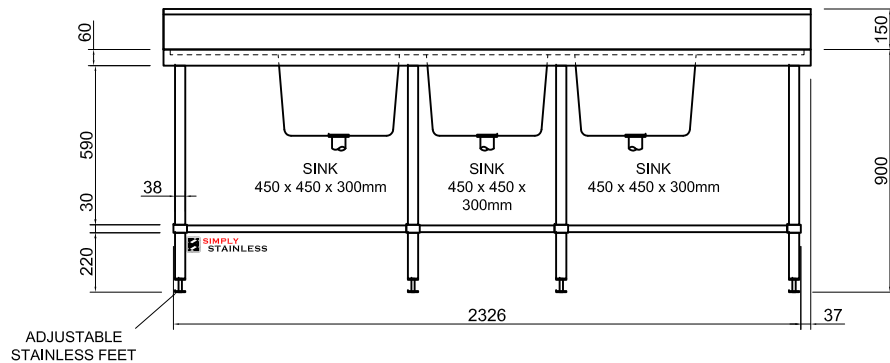
FRONT ELEVATION
