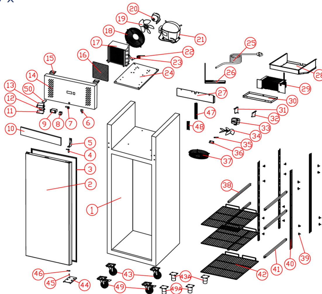
EXPLODED DIAGRAM XURC600SFV
