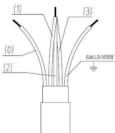
V220-240/2 SINGLE-PHASE
