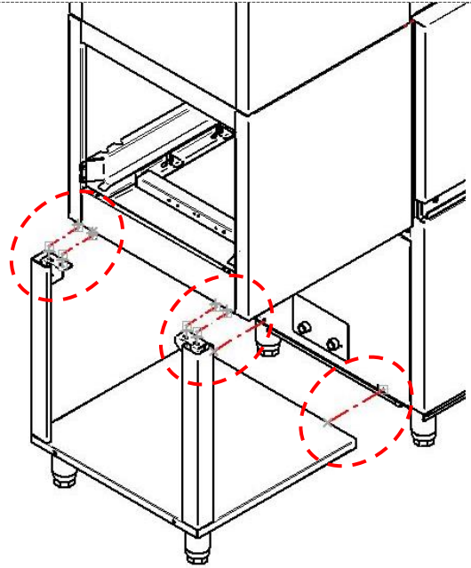
Image 21.- Tray attachment
