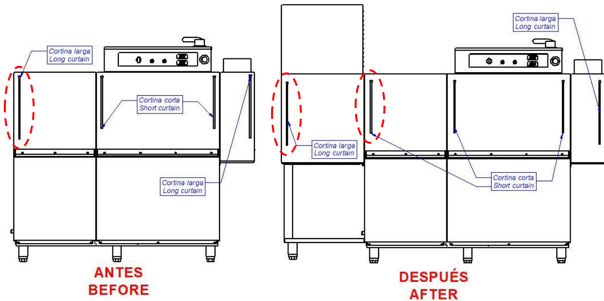
Image 22.- Curtains placement
