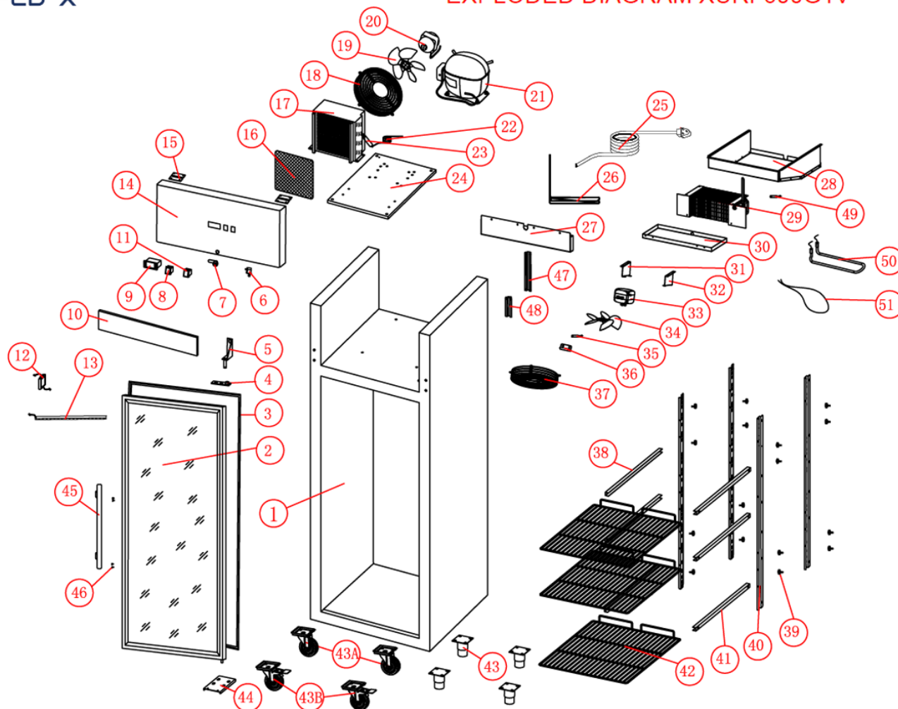
EXPLODED DIAGRAM XURF600G1V
