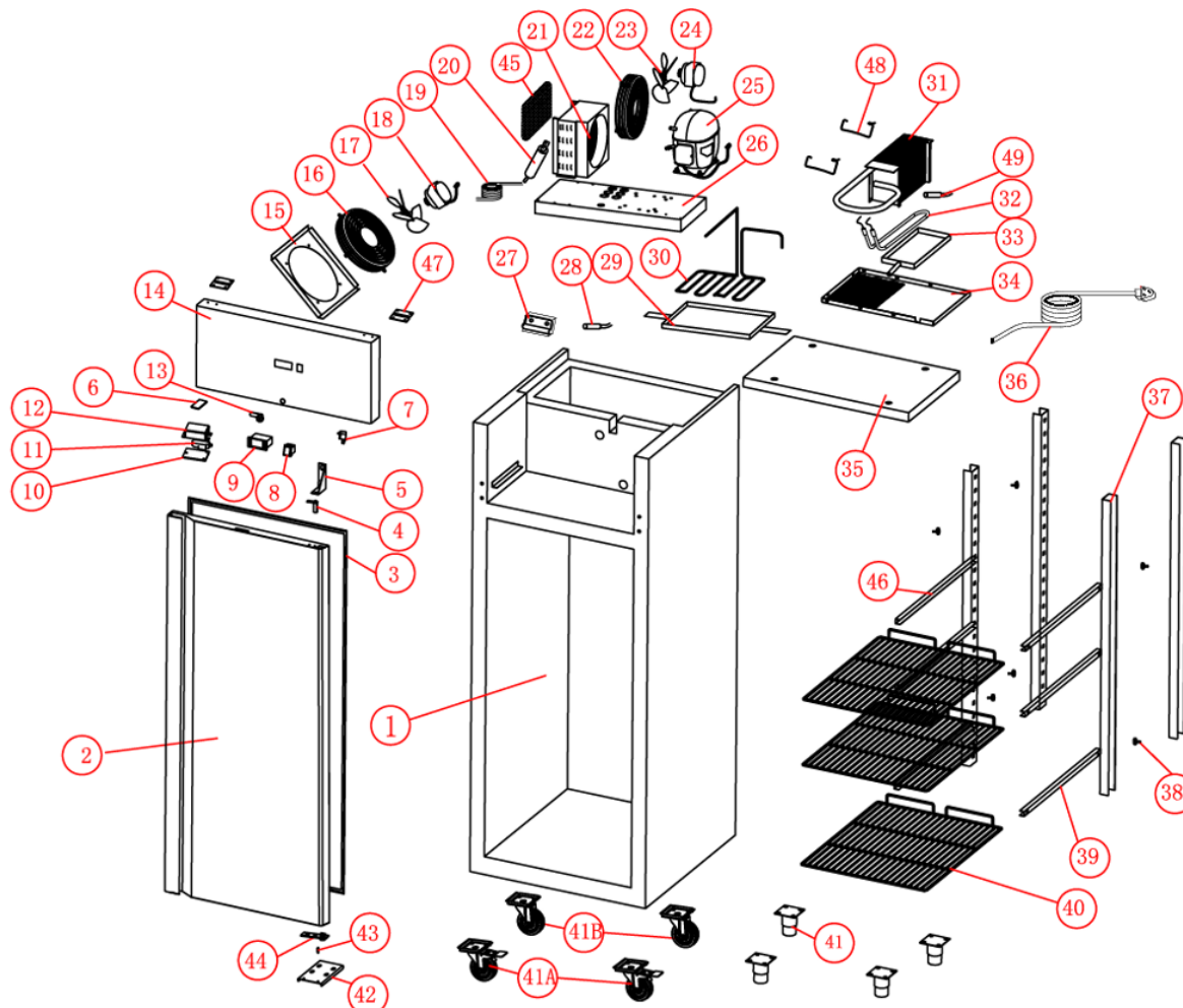
EXPLODED DIAGRAM XURF650SFV
