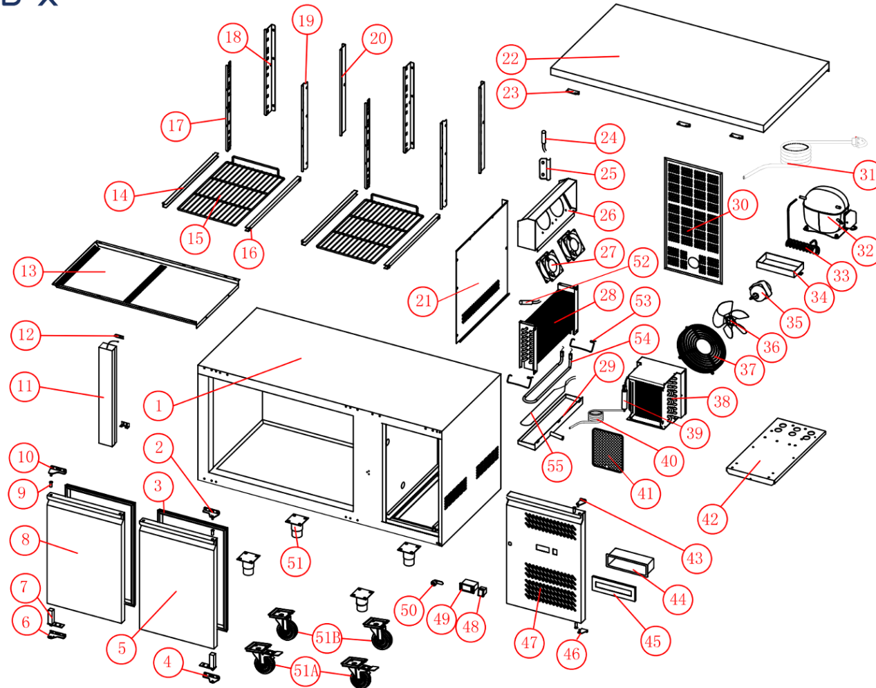
XUB7F13S2V EXPLODED DIAGRAM
