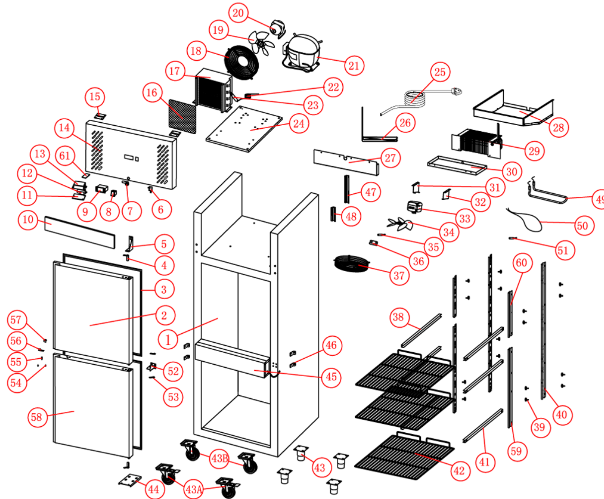
EXPLODED DIAGRAM XURF600S1V
