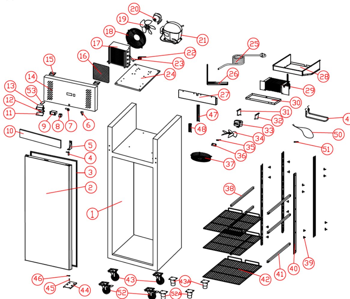
EXPLODED DIAGRAM XURF600SFV
