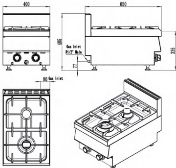
AT65G2B-C
