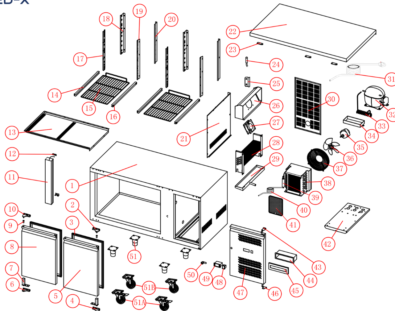
XUB7C13S2V EXPLODED DIAGRAM
