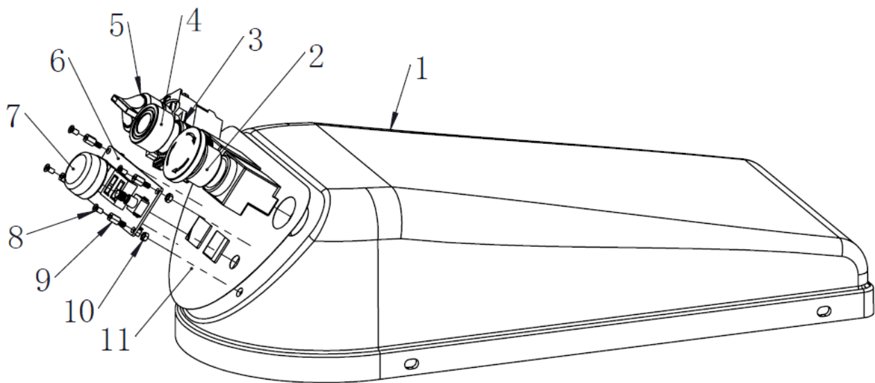
FIGURE 2 Top Cover
