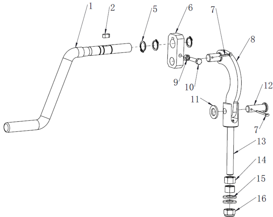
FIGURE 5 LIFT HANDLE
