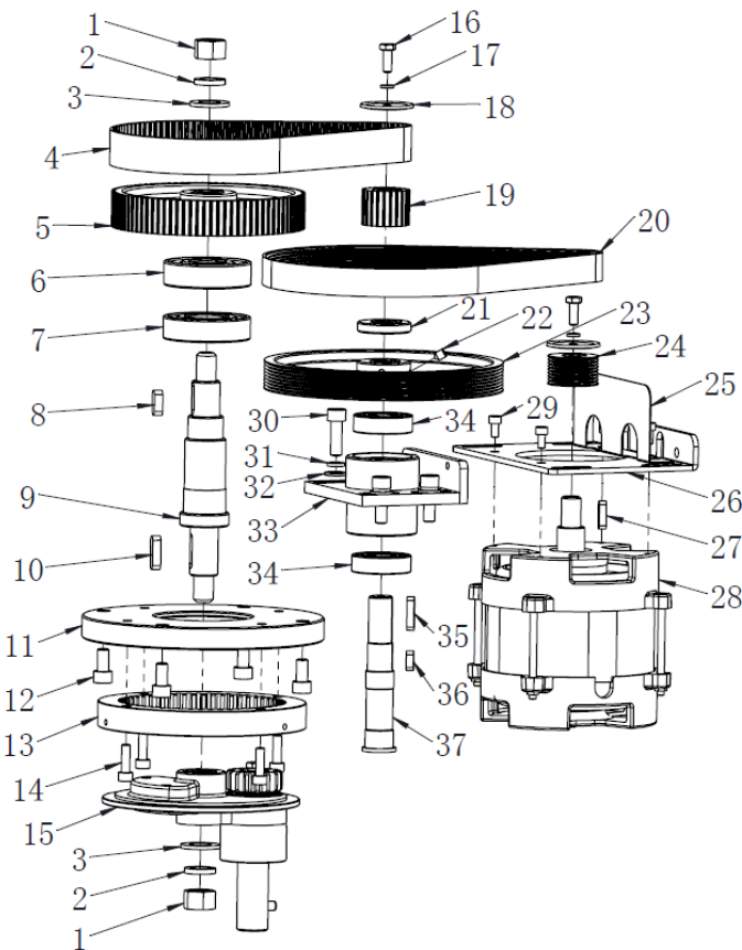
FIGURE 3 DRIVE SYSTEM
