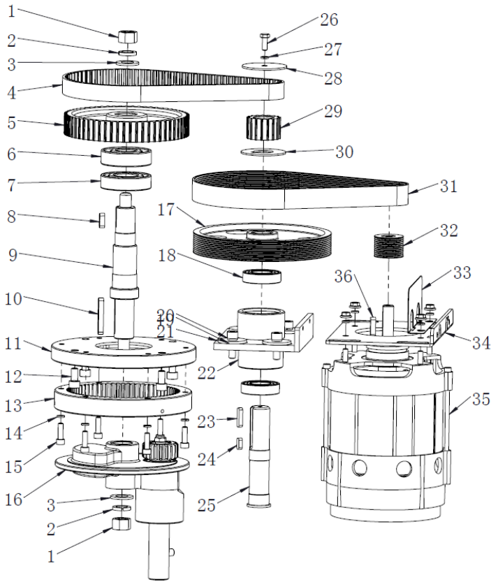
FIGURE 3 DRIVE SYSTEM
