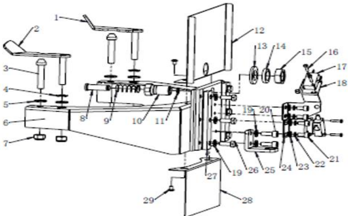
FIGURE 4 ARM
