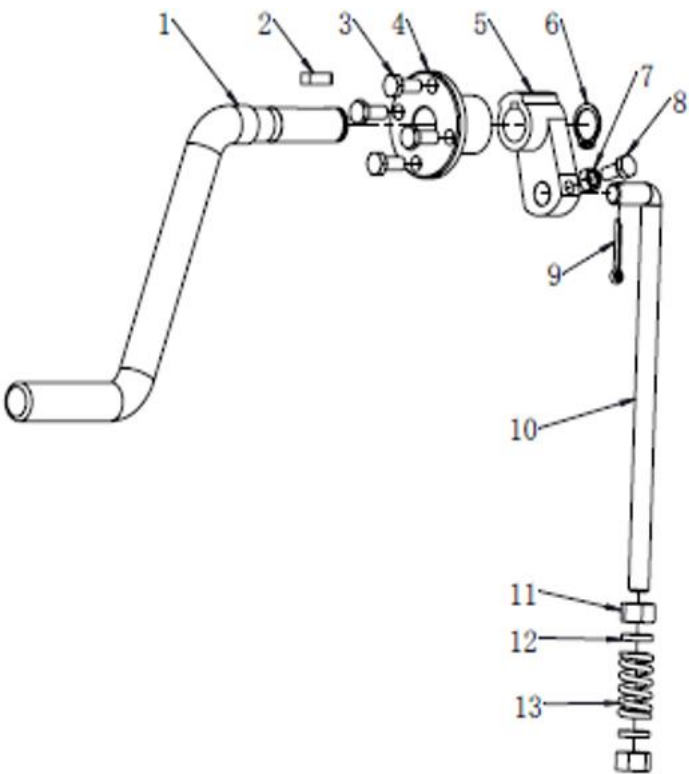
FIGURE 5 LIFT HANDLE
