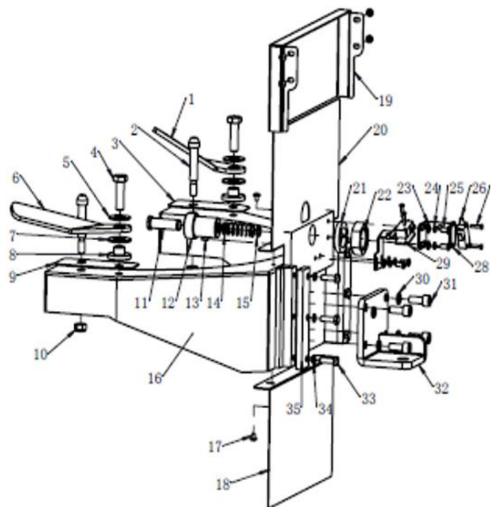
FIGURE 4 ARM
