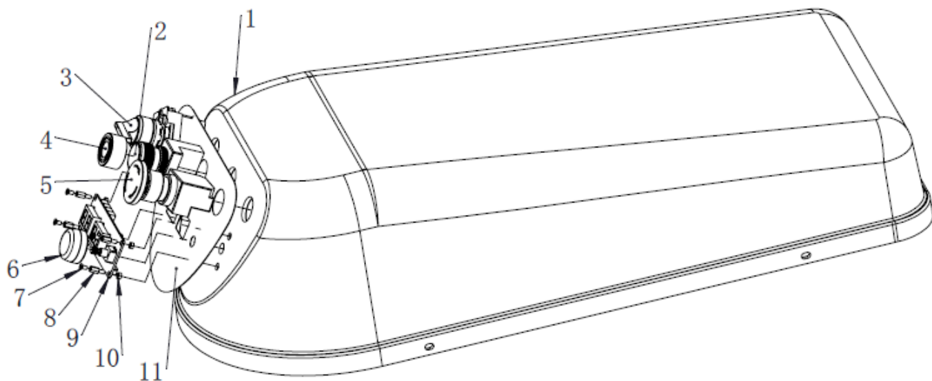
FIGURE 2 Top Cover
