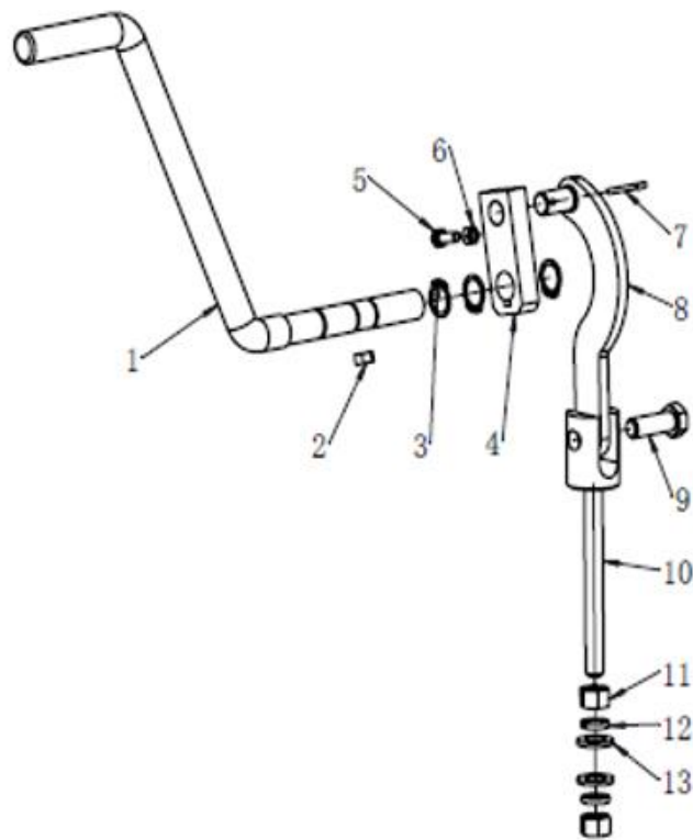
FIGURE 5 LIFT HANDLE
