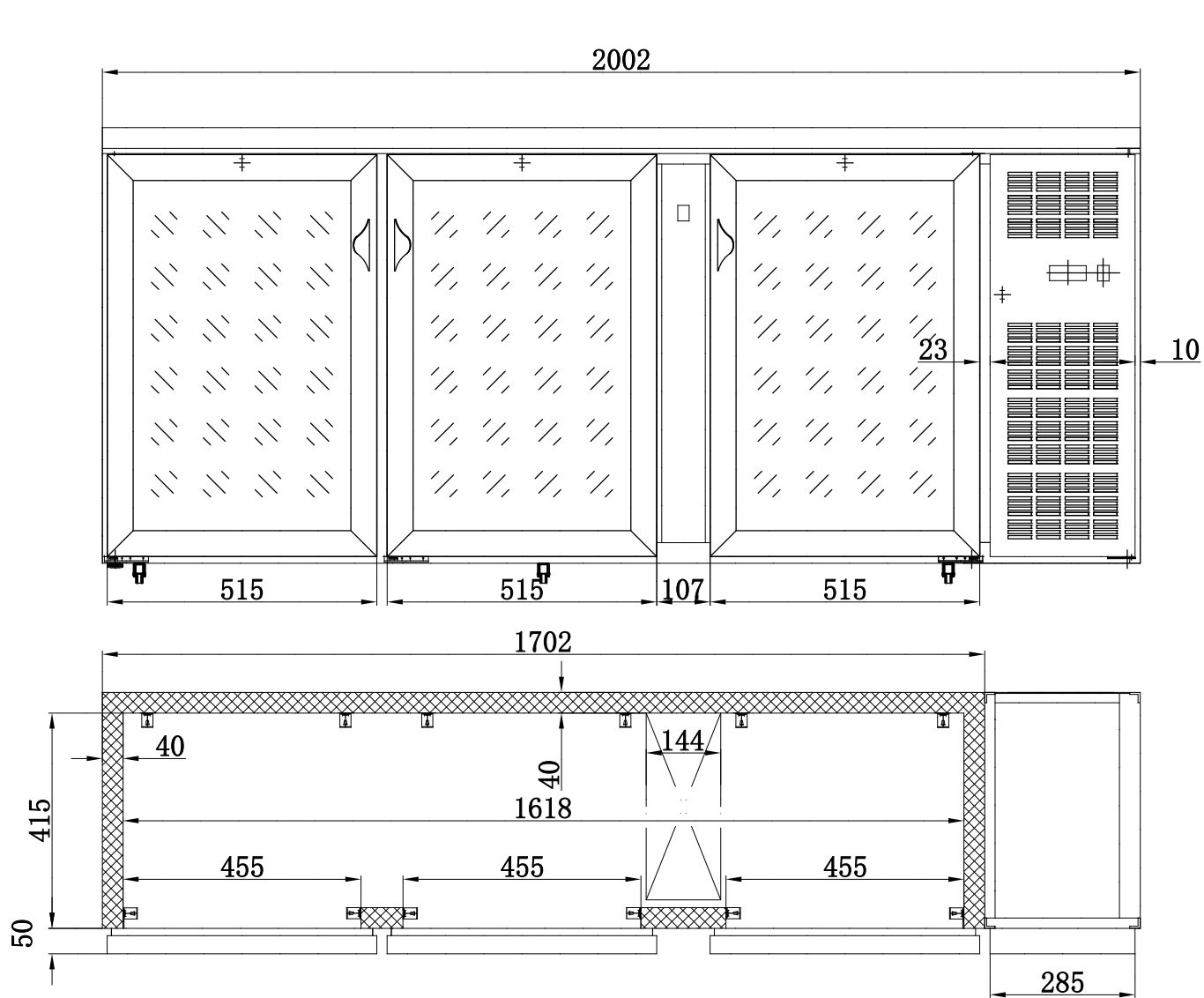
OUTSIDE DRAWING OF BC3100G
