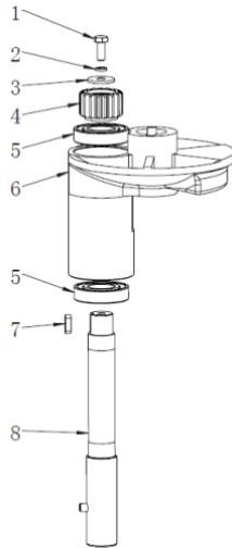
FIGURE 6 TURNING PLATE AND MIXING AXLE
