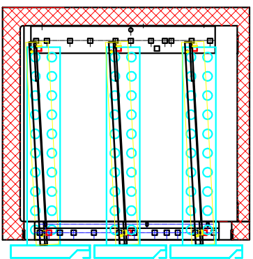
installation diagram
