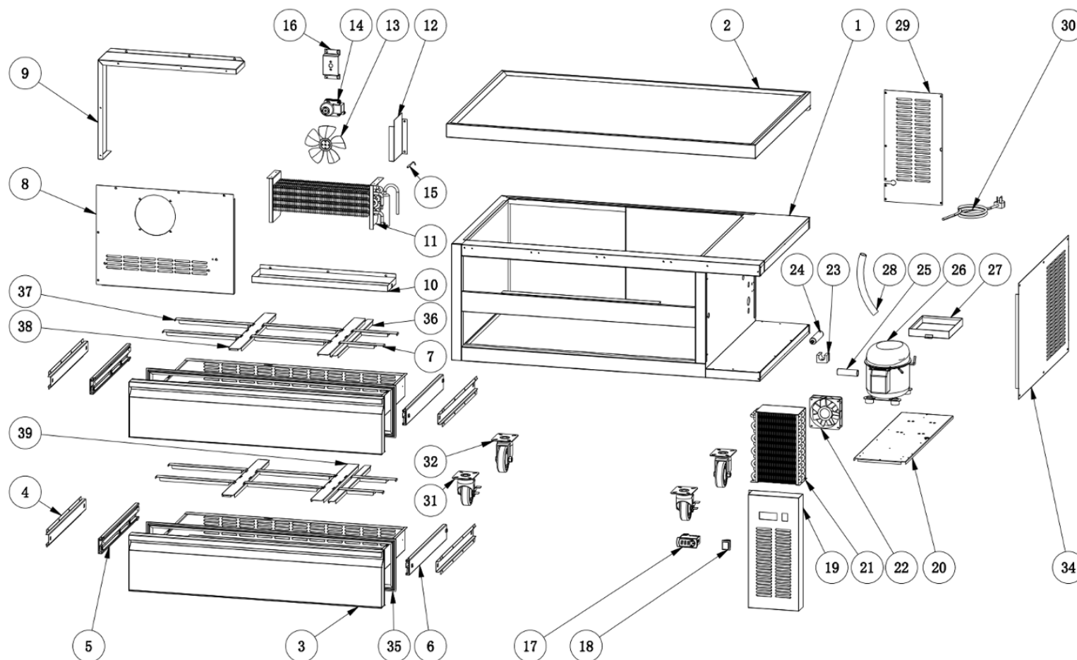
EXPLODED DIAGRAM XCB-48
