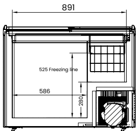
WD256G
