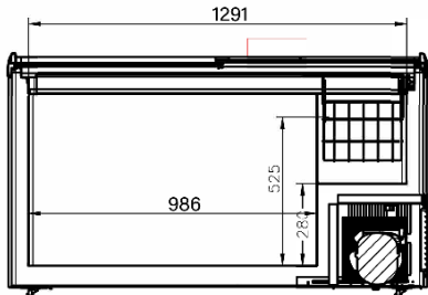
WD396G
