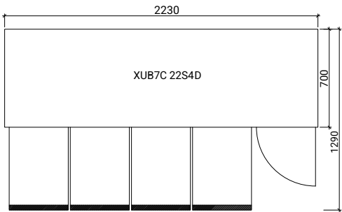
Front Side
