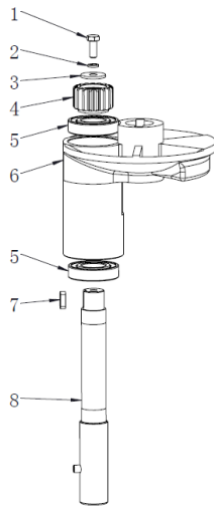
FIGURE 6 TURNING PLATE AND MIXING AXLE
