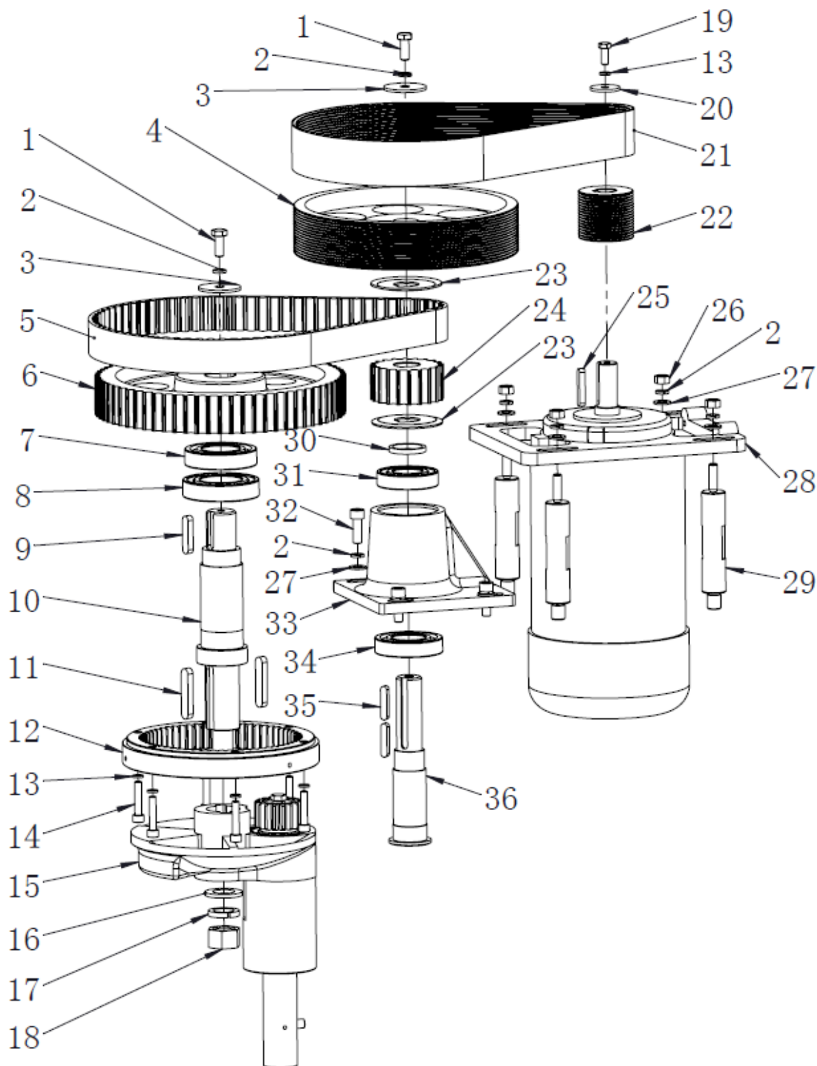
FIGURE 3 DRIVE SYSTEM
