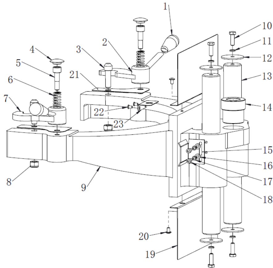
FIGURE 4 ARM
