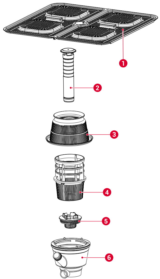
Fig. 4: Machine filters
