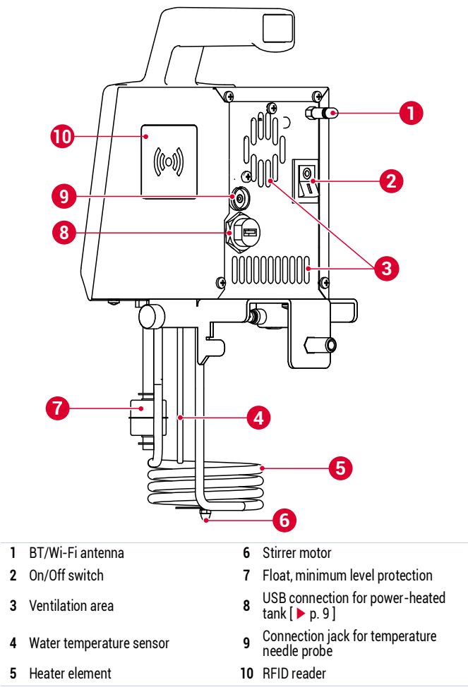
Fig. 1: SmartVide X/XL, main components, part 1
