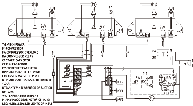
ELECTRIC WIRING DIAGRAM(FABIGANI-3S )
