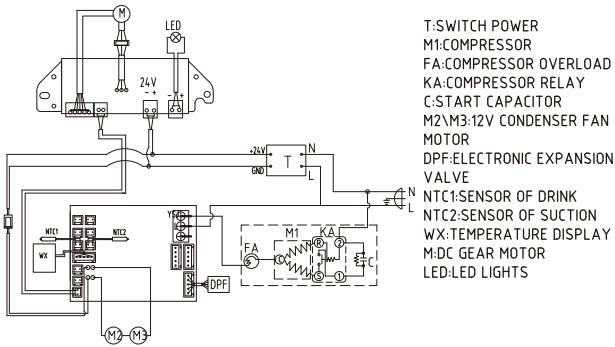
ELECTRIC WIRING DIAGRAM( FABIGANI-2S )
