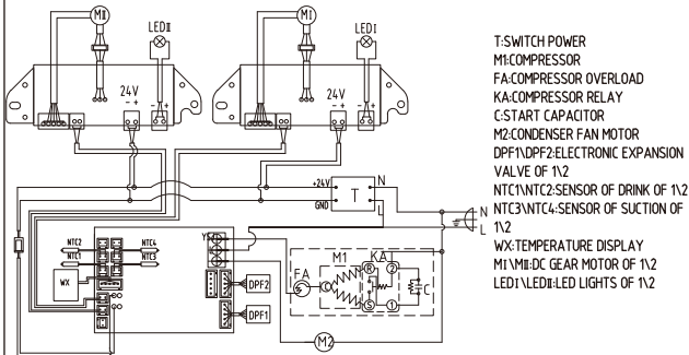
ELECTRIC WIRING DIAGRAM( FABIGANI-2S )
