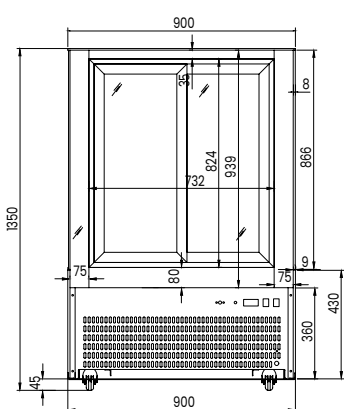
H-SF830V
