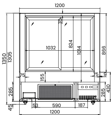
SF840V
