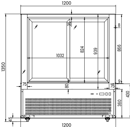
H-SF840V
