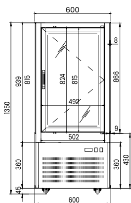
H-SF820V
