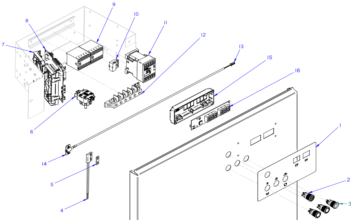
FIGURE 4 CONTROL PANEL
