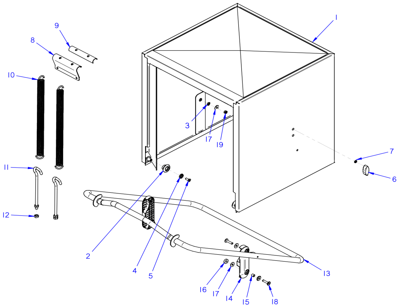
FIGURE 2 HOOD
