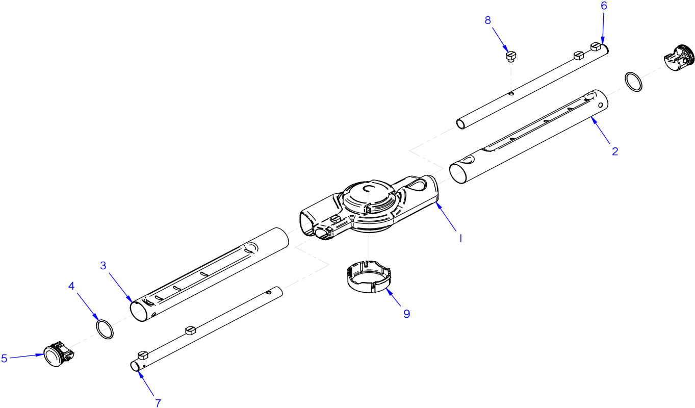
FIGURE 8 SS DISPENSER(OPTIONAL)
