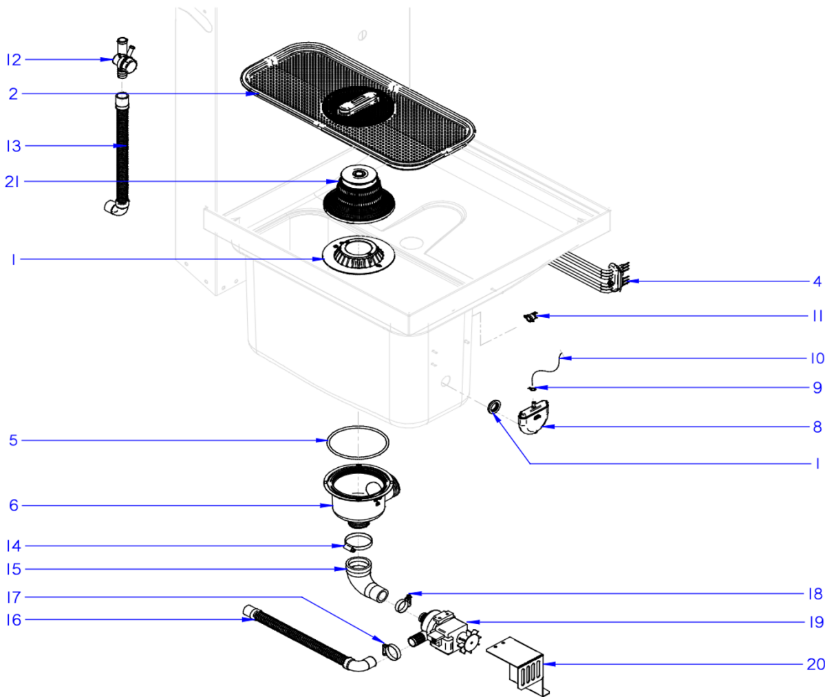
FIGURE 3 TANK PARTS
