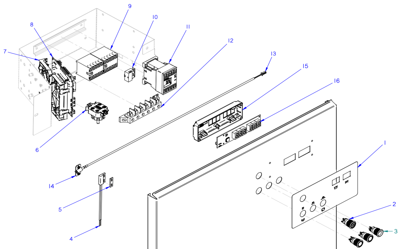
FIGURE 4 CONTROL PANEL
