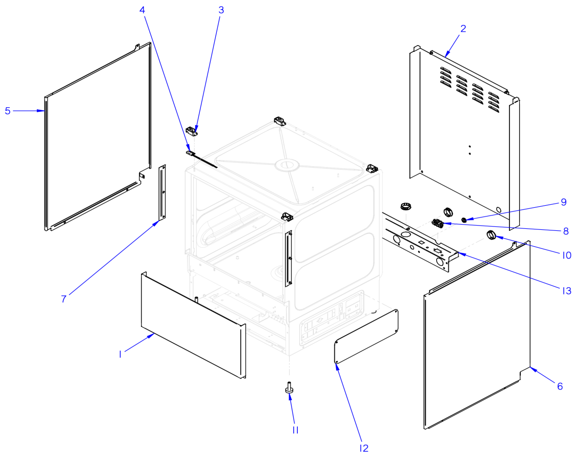
FIGURE 1 PANELS OF THE MACHINE
