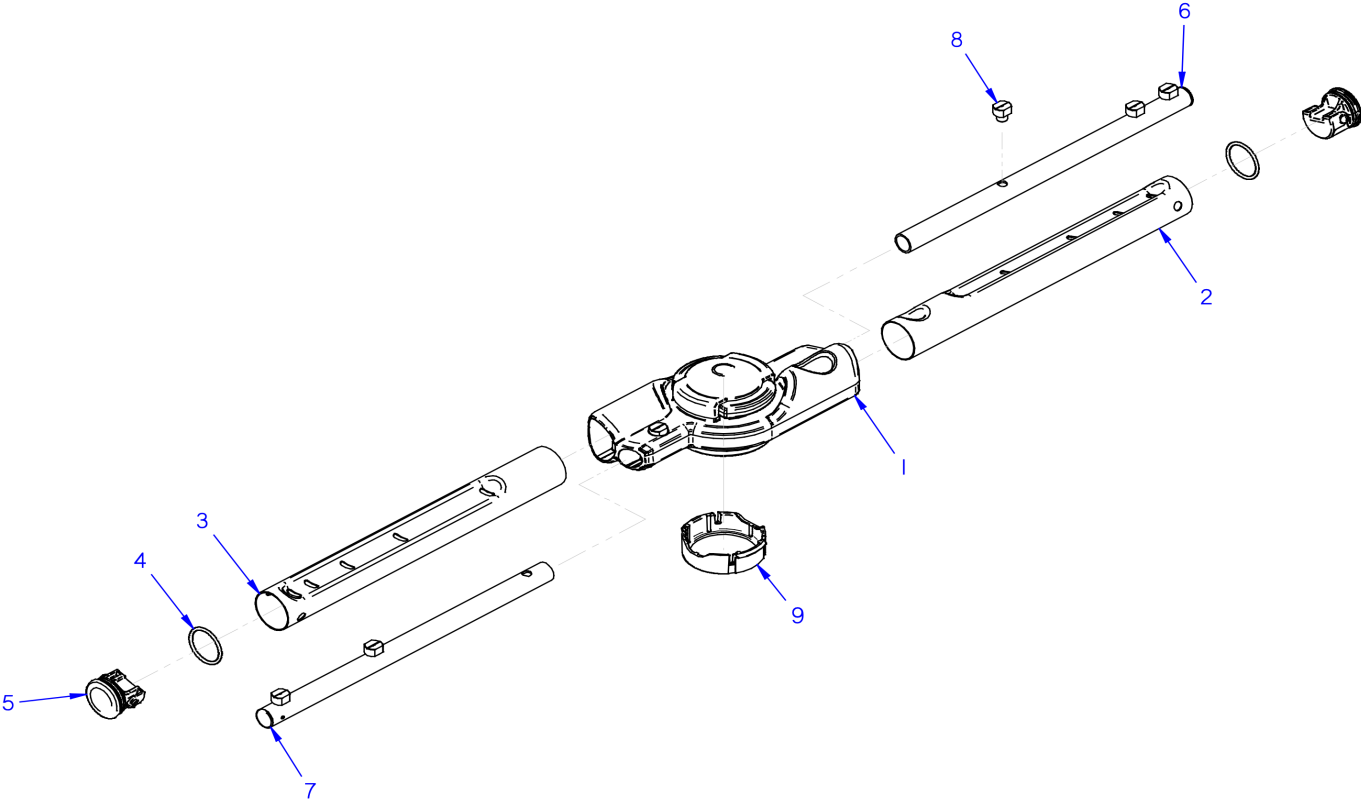
FIGURE 8 SS DISPENSER(OPTIONAL)
