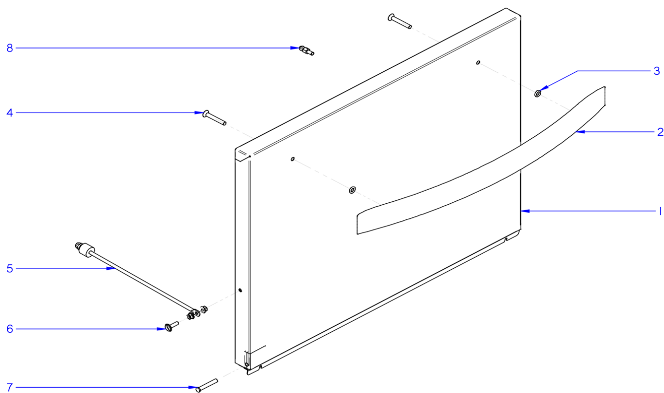
FIGURE 2 DOORS
