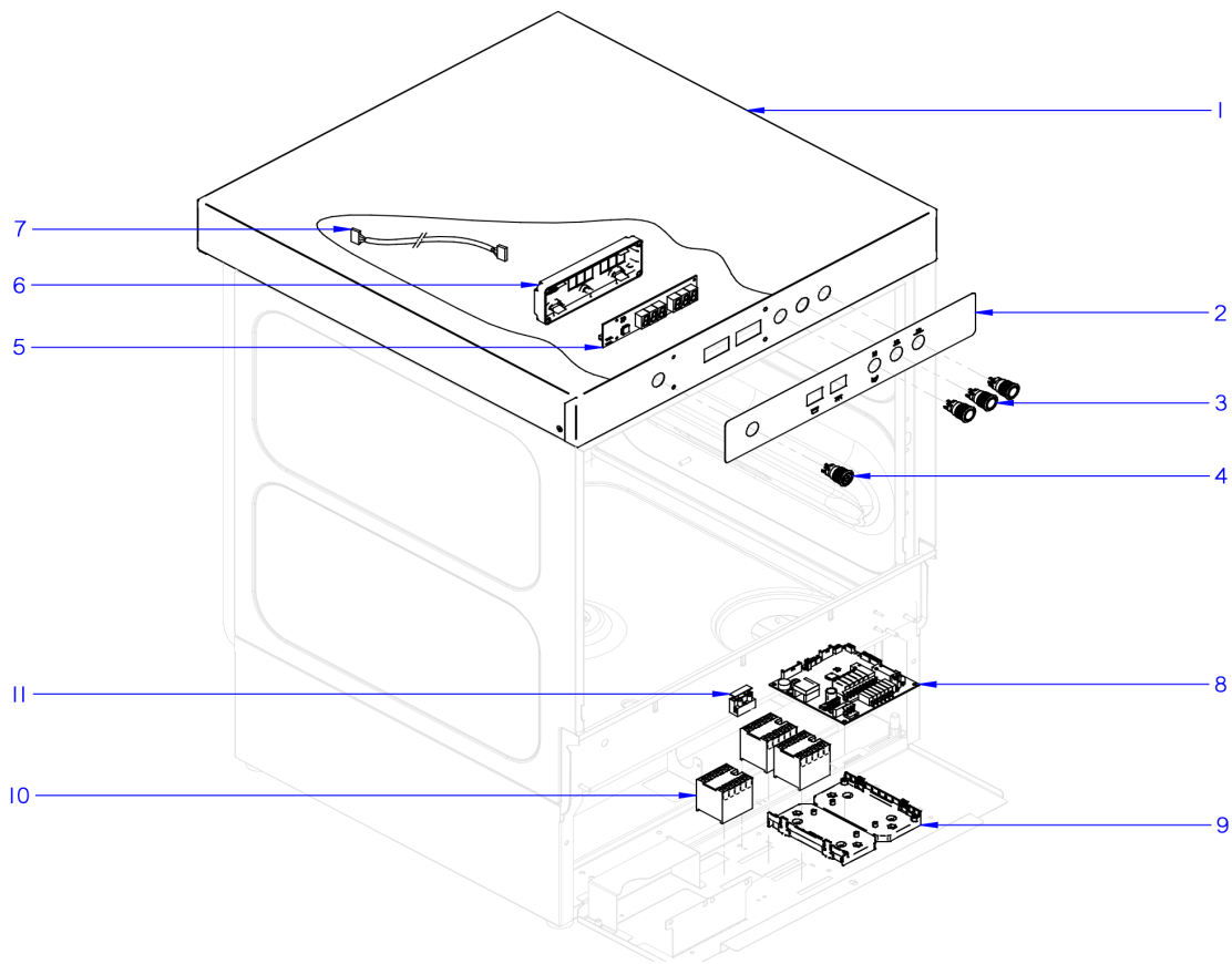
FIGURE 4 CONTROL PANEL
