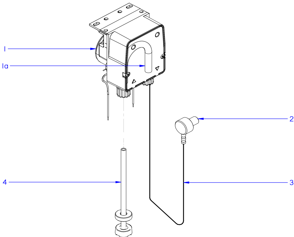
FIGURE 7 DET.DISPENSER
