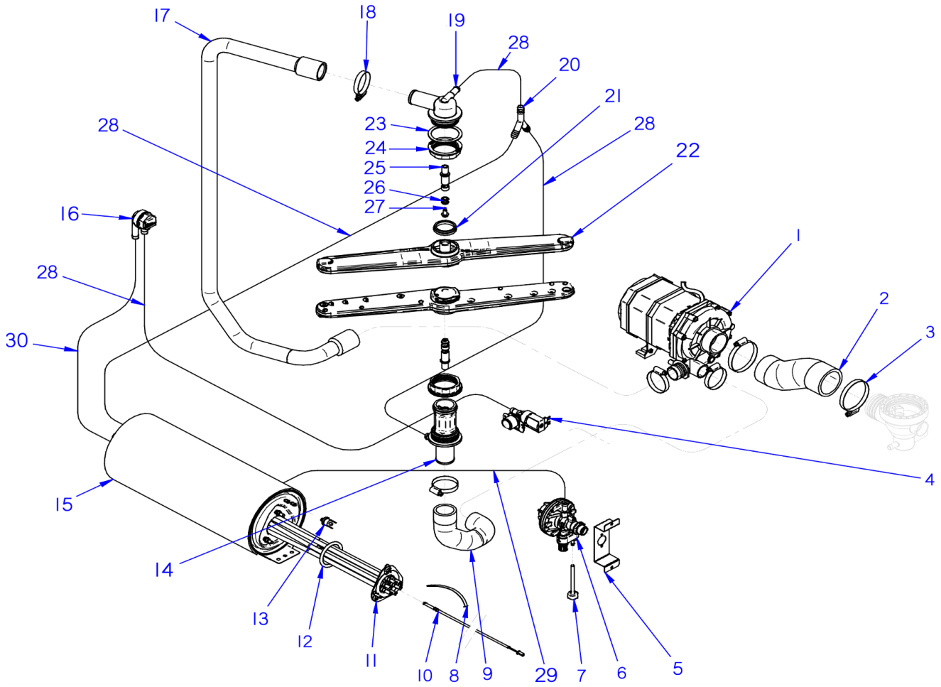
FIGURE 5 HYDRAULIC STSYEM
