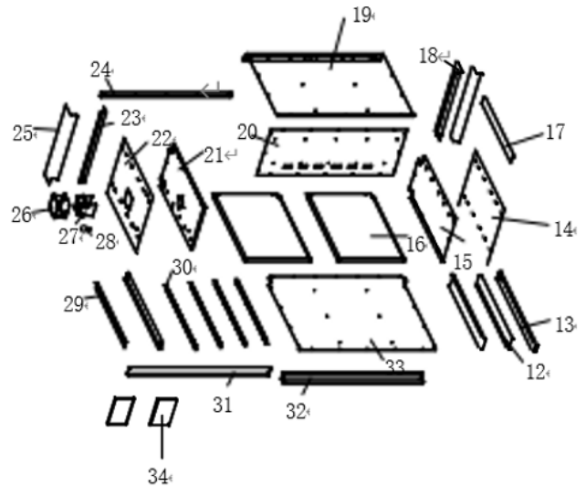
Inner Case
