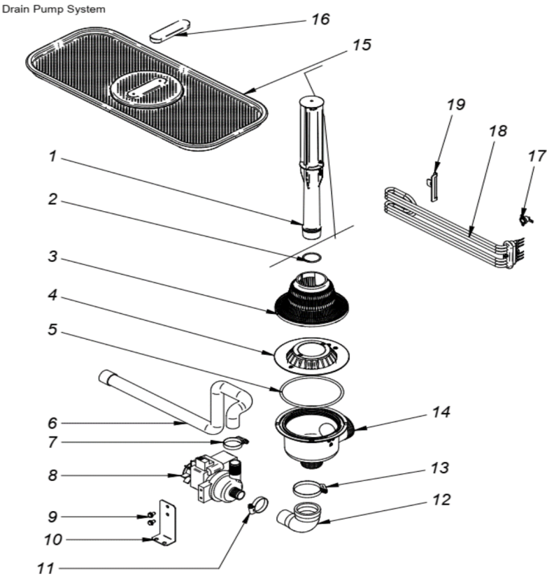
Drain Pump System
