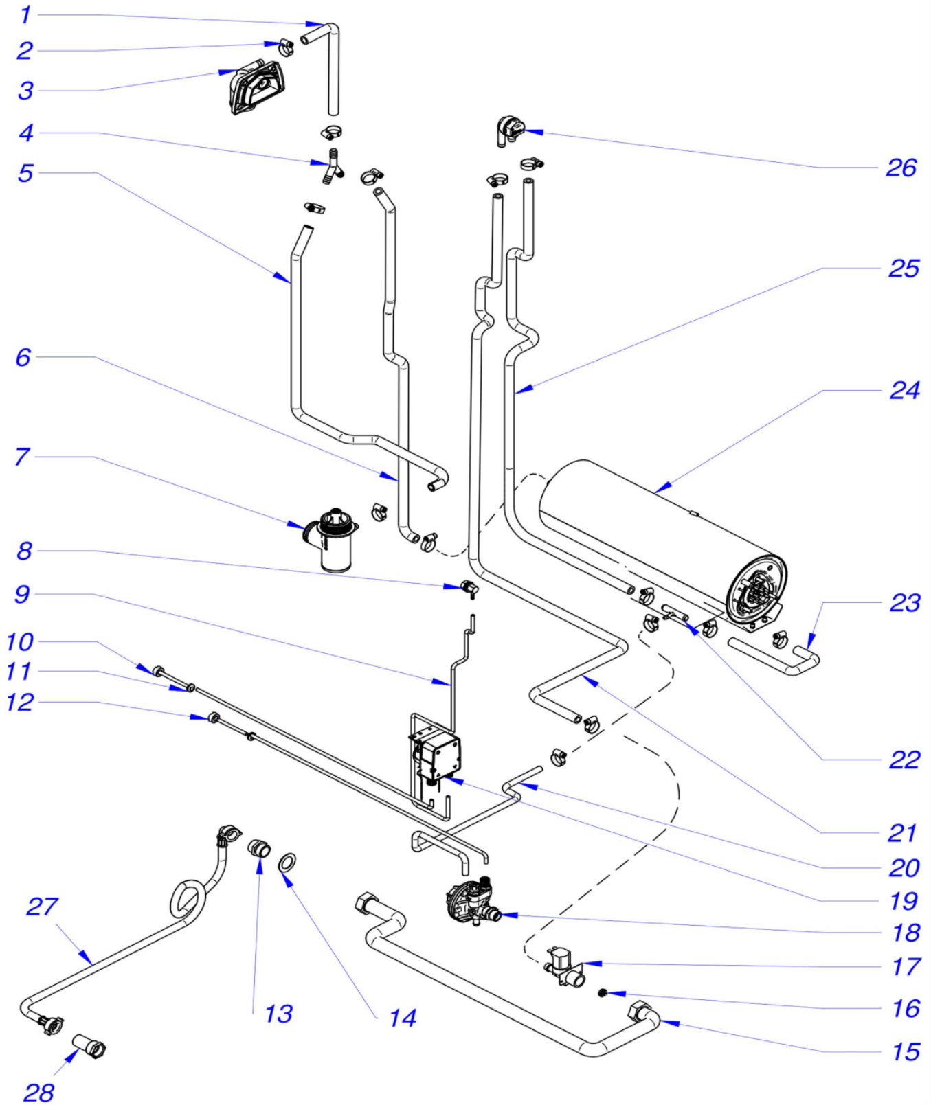
FIGURE 4 HYDRULIC SYSTEM
