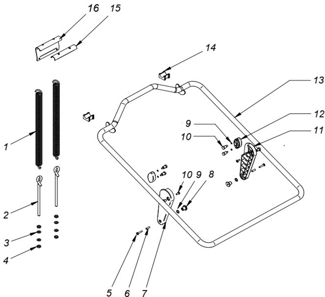
FIGURE 2 TILTING SYSTEM
