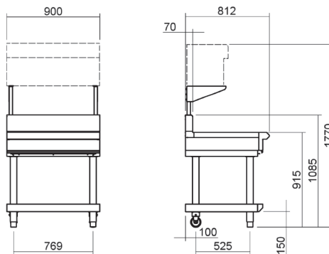
B90S-LS Leg Stand
