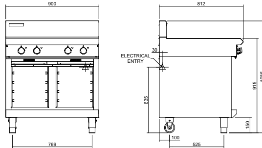
IN514R3, IN514R5
