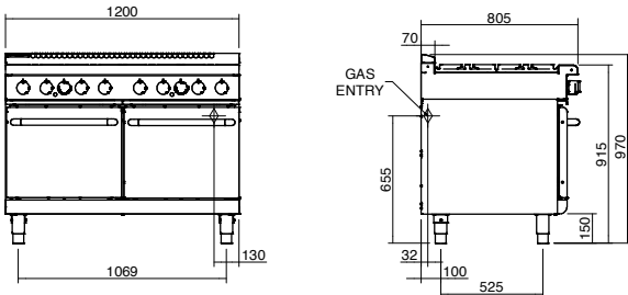
RNLB8820G
