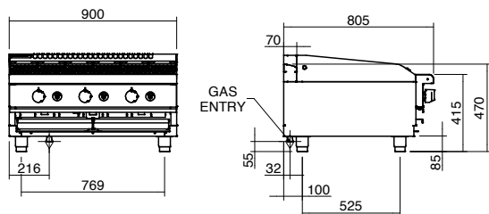
CHLB8900G-LS/CD
