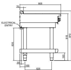
INLB8100F
