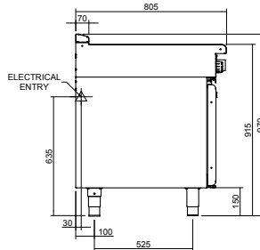
INLB8100R3 / INLB8100R5
