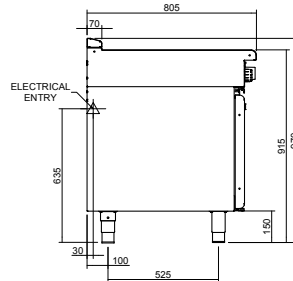
INLB8200R3 / INLB8200R5
