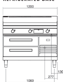
GP8120E-RB REFRIGERATED BASE
