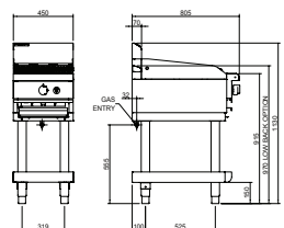
CH8450G-LS/CB
