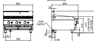
CH8900G-B
