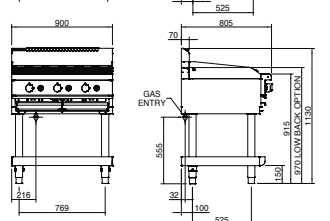
CH8900G-LS/CB
