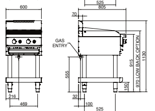
CH8600G-LS/CB
