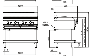
CH8600G
