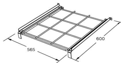
Internal Grid
