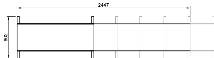
Plan View
