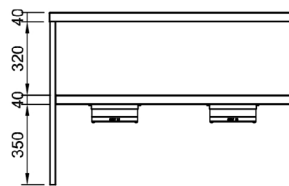
Front Elevation
