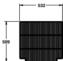
SHELF DETAIL
