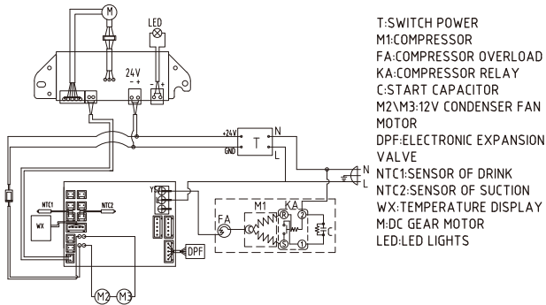
ELECTRIC WIRING DIAGRAM( FABIGANI-2S )
