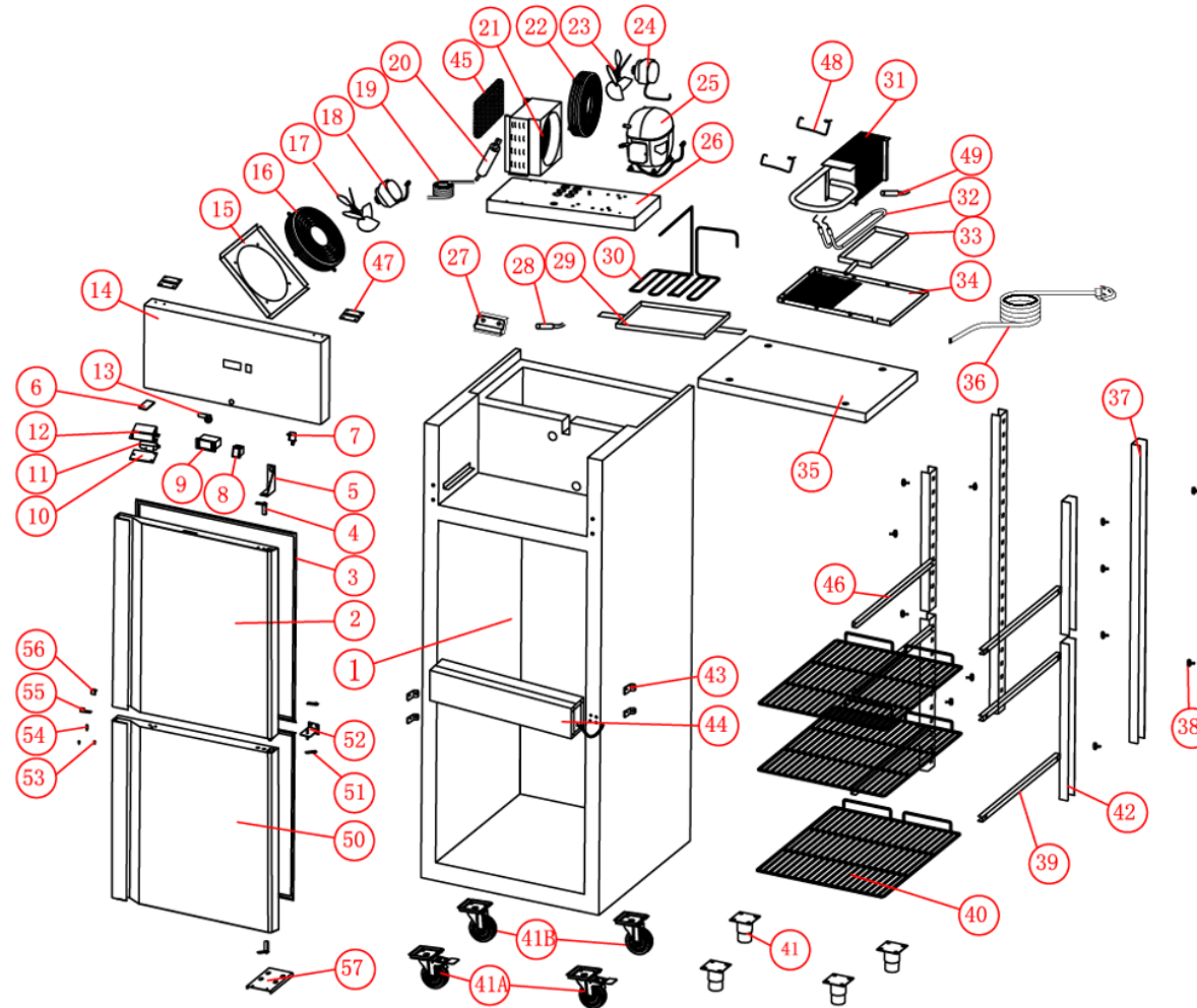
EXPLODED DIAGRAM XURF650S1V
