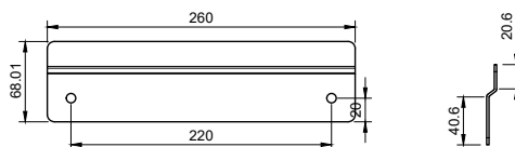
Mounting Bracket
