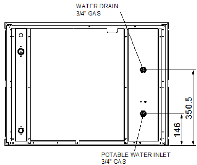
Water Cooled
