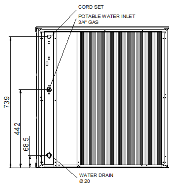
Air Cooled
