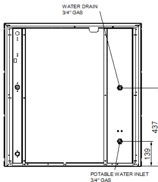
Water Cooled
