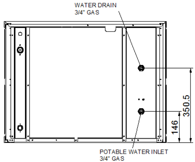
Water Cooled
