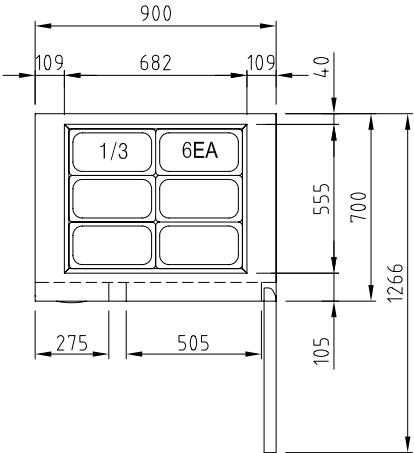
PLAN VIEW
