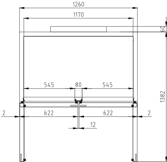
PLAN VIEW (unit : mm)
